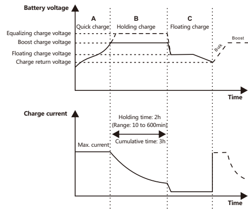
Figure 1-5 Battery charging stages curve graph
