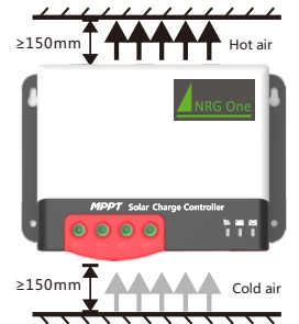
Figure 2.1 Installation and Heat Dissipation
