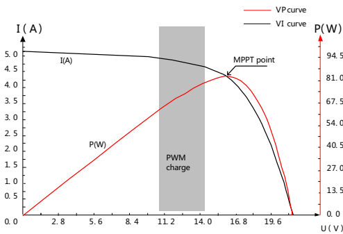
Figure 1-2 Solar panel output characteristics curve
